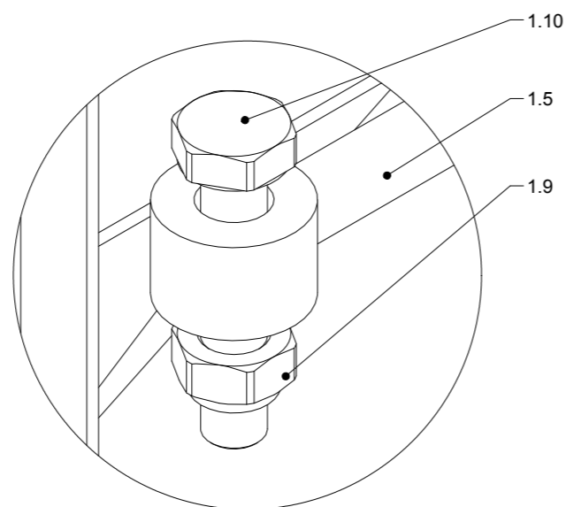
DETAIL C (1 : 1)
