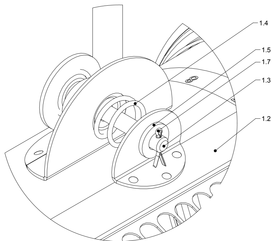
DETAIL A (1 : 1)
