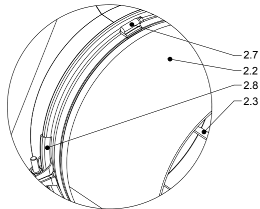
DETAIL C (1 : 5)
