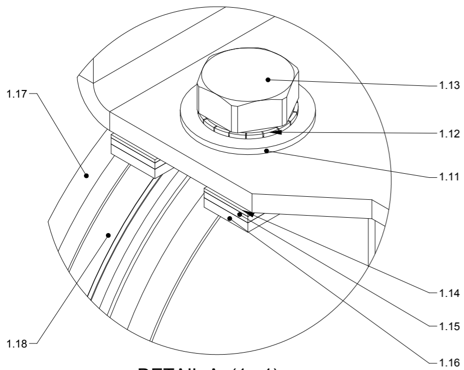
DETAIL A (1 : 1)
