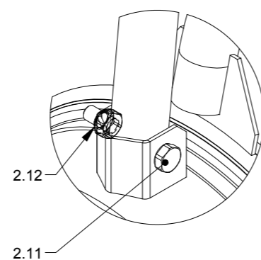
DETAIL C (1 : 2)
