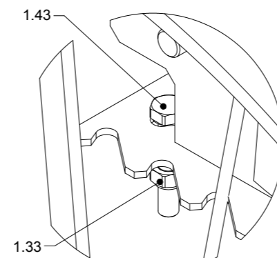
DETAIL F (1 : 2)
